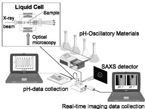
Figure 2. Experimental set-up for the dynamic pH studies.
